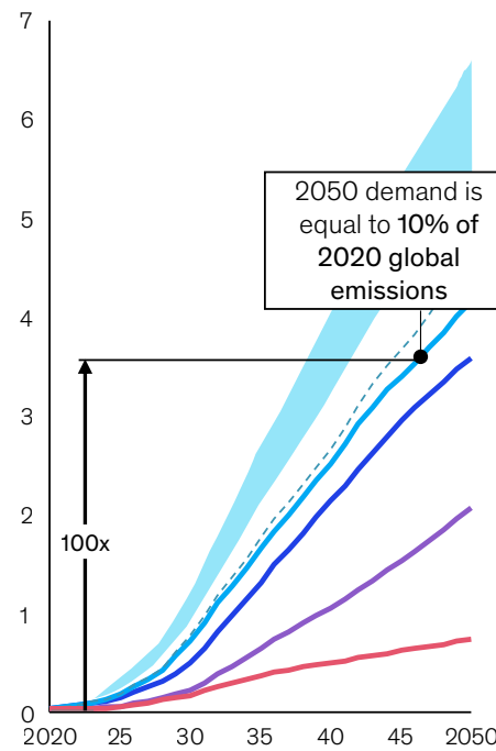
Global CCUS uptake by scenario Gt CO 2
