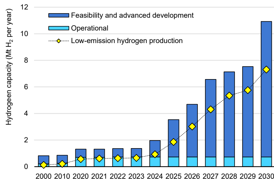
Past and planned capacity of CCUS-equipped hydrogen production facilities, 2000-2030
